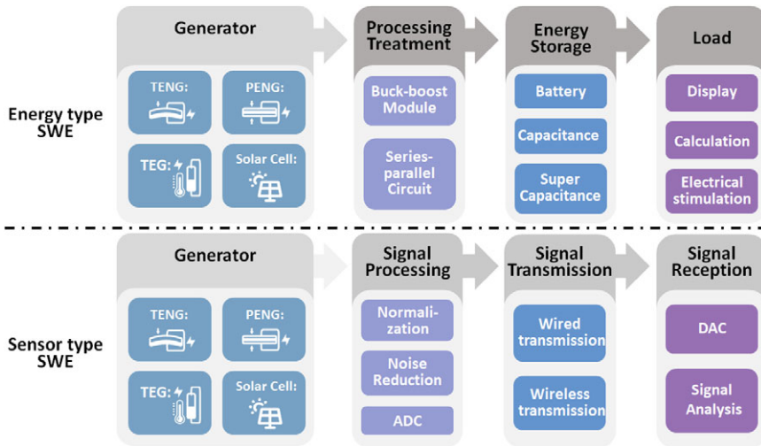
Figure 2. Energy management of energy type SWE and sensor type SWE. According to the difference in the form of energy utilization, SWE can be divided into energy type SWE and sensor type SWE.
