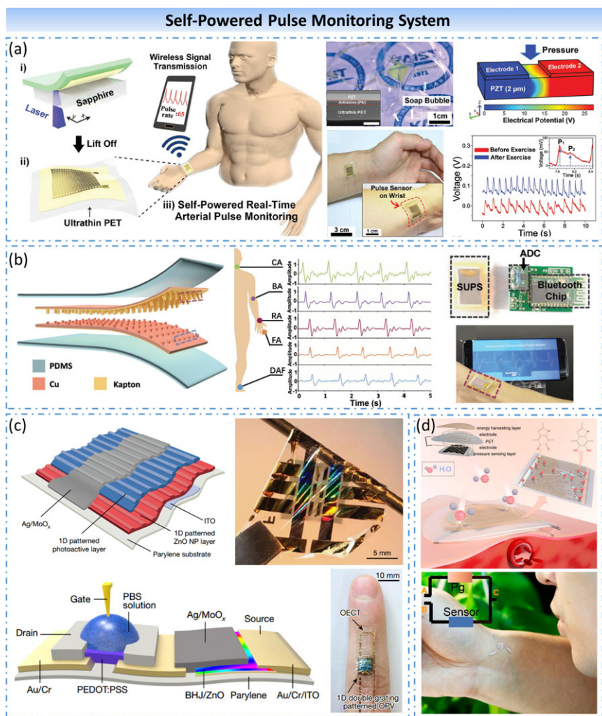
Figure 7. Self-powered pulse monitoring system. (a) Ultrathin epidermal piezoelectric sensor for real-time arterial pulse monitoring. (b) Flexible self-powered ultrasensitive pulse sensor based on triboelectric effect. (c) Self-powered ultra-flexible biosensor based on nanograting-patterned organic photovoltaics. (d) Moisture-driven flexible multifunctional sensing system based on flexible piezoresistive sensor and moisture-enabled power generator.
