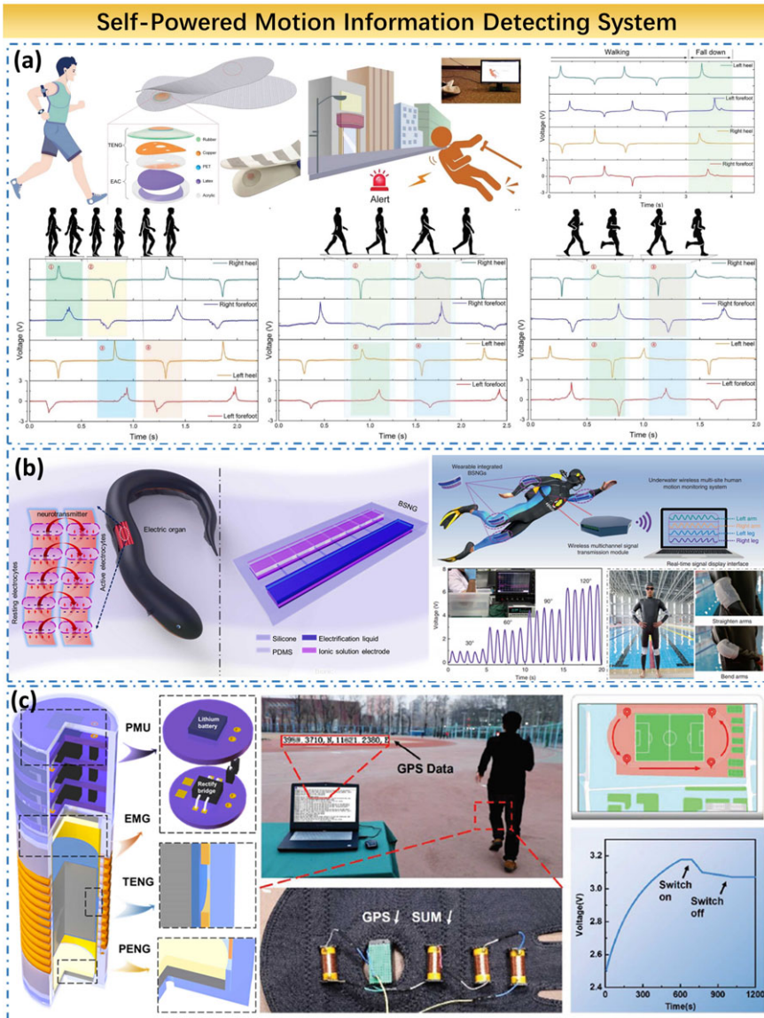
Figure 10. Self-powered motion information detecting system. (a) Multifunctional gait monitoring system based on triboelectric nanogenerator. (b) Underwater wireless multisite motion monitoring system based on bionic stretchable nanogenerators. (c) Self-powered GPS location system based on battery-like self-charge universal modules.
