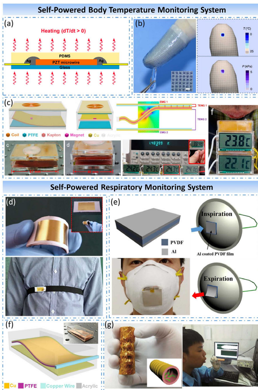
Figure 6. Self-powered body temperature monitor system and self-powered respiratory monitor system.
