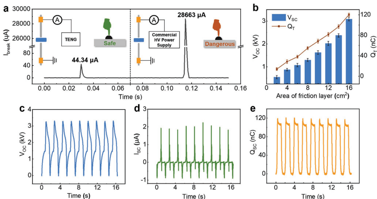
Figure 2. Electrical characterization of TENG. a) Breakdown current values of the DED actuated by TENG (16 \text{cm}^2 area) and commercial HV power, respectively, and schematic diagram of test connection. b) Open-circuit voltage and transfer charge of the TENG under different friction layer area. c) Open-circuit voltage of the TENG with area of 16 \text{cm}^2 . d) Short circuit current of the TENG with area of 16 \text{cm}^2 . e) Transferred charge of the TENG with area of 16 \text{cm}^2 .
