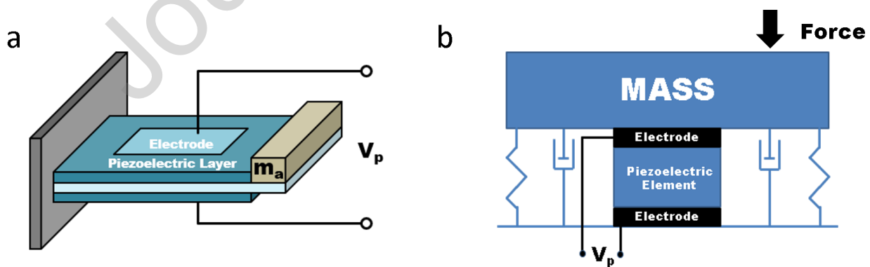
Figure 11. Piezoelectric harvester model. (a) Cantilever beam (common piezoelectric-based power generator). (b)
