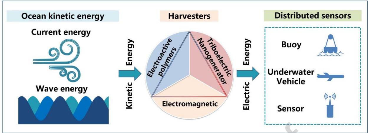
Figure 4: Schematic of OKE harvesters for powering distributed sensors.
