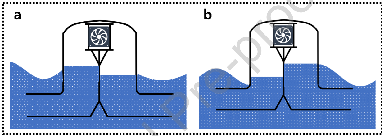
Figure 7: Double chambered backward bent duct buoy (BBDB) (adapted from [114]).
