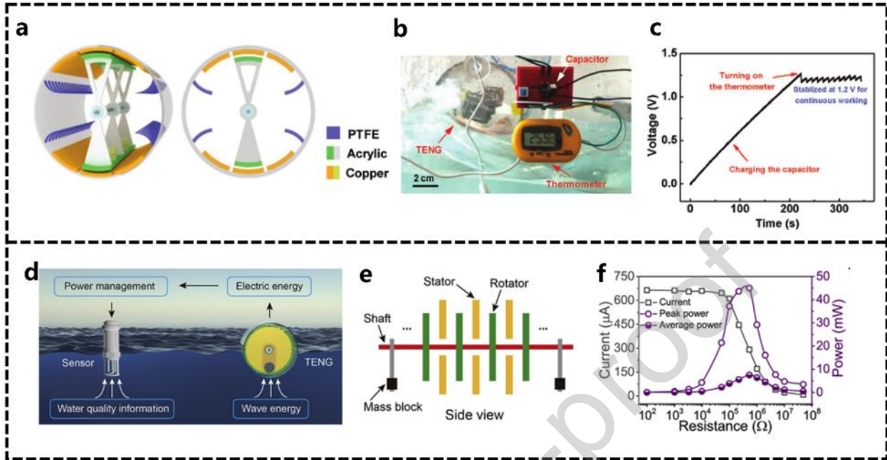
Figure 17: (a) Schematic diagram of the 3D structure and cross-section for the SS-TENG. (b) Photograph of a digital thermometer powered by the SS-TENG and (c) the charging process for a capacitor of 220 \mu\text{F} to power the thermometer under the wave conditions of 10 cm and 1.2 Hz. (d) Schematic diagram of the water quality monitoring system and the illustration of the side view (e) of the TD-TENG. (f) The peak current, peak power and average power of the TD-TENG under various loads in water. (a-c) Reproduced with permission from Wiley [219]. (d-f) Reproduced with permission from Elsevier [158].
