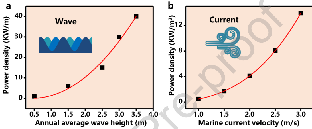
Figure 3: Relative power density of (a) ocean wave with different wave heights and (b) marine current with different current velocities [76, 77].
