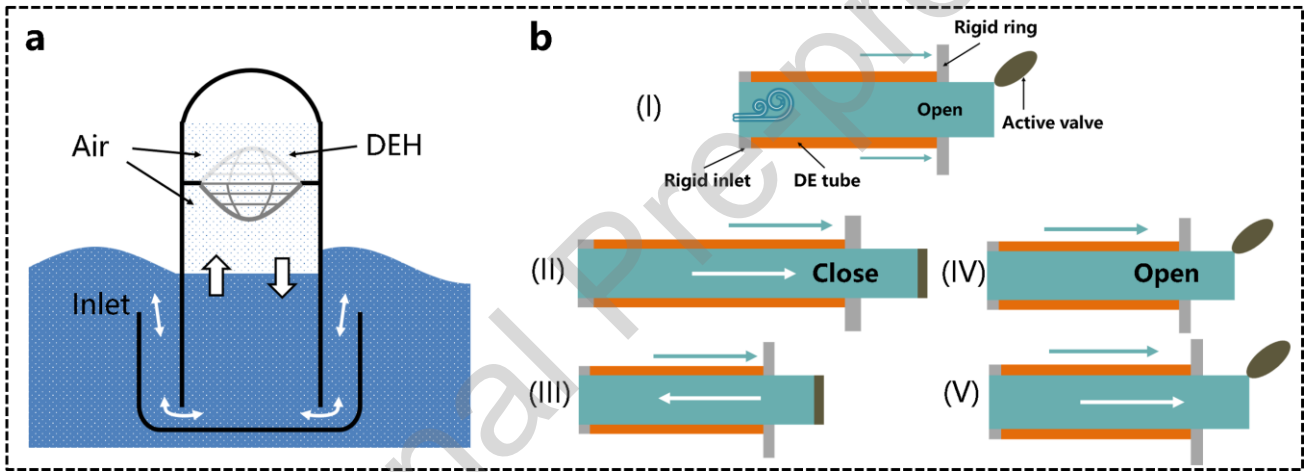
Figure 10: (a) Pseudo-OWC-type DE WEH. (b) Mechanical design and working principle of the flow energy converter in the opened and closed state.
