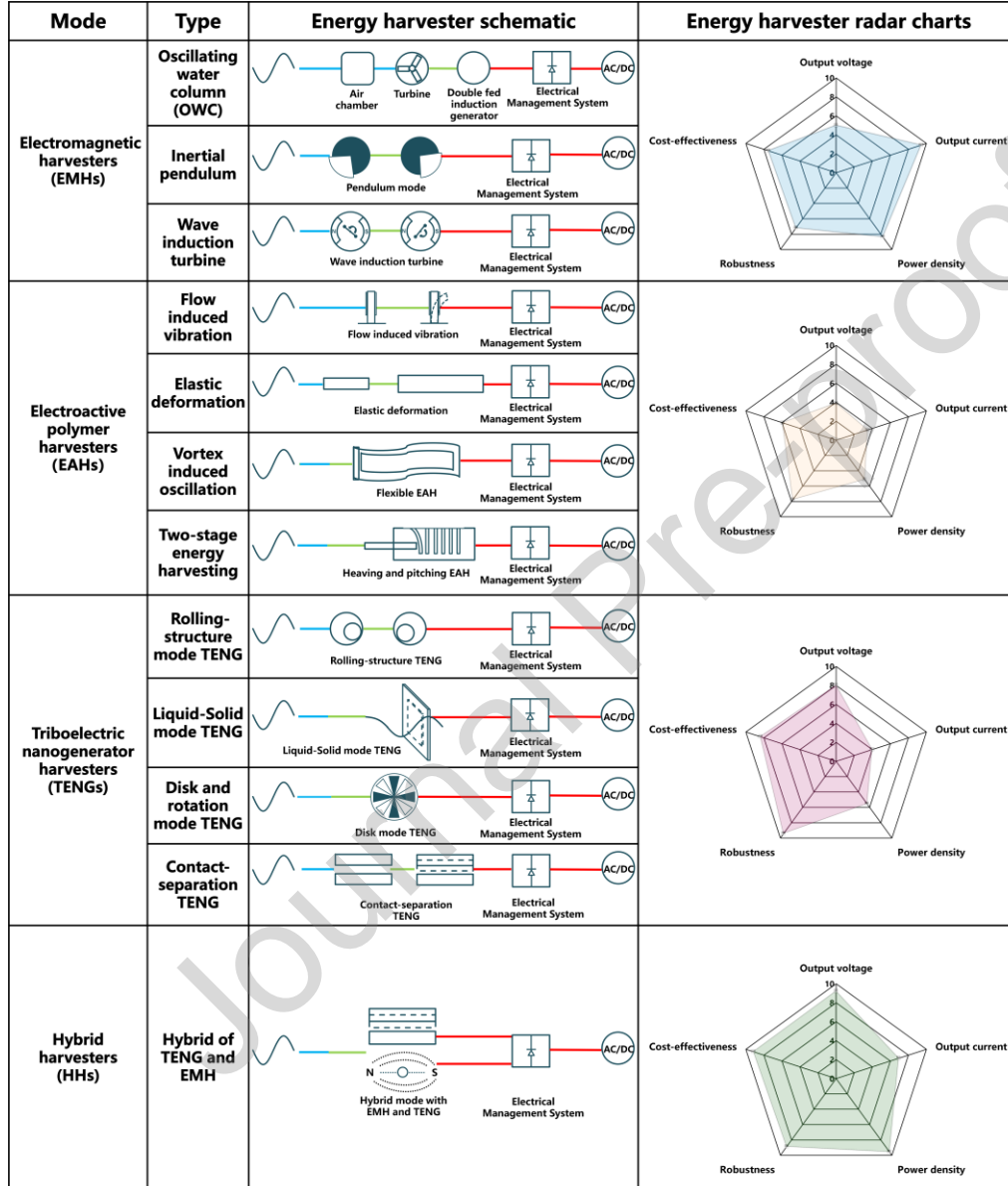
Figure 21: Flow-machine-electrical conversion and the characteristics of the various OKEHs: OWC [103], inertial pendulum [102, 105], wave induction turbine [96], flow induced vibration [112, 113, 144, 146, 231], dielectric elastomer [111, 113], vortex induced oscillation [137], two-stage energy harvesting [232], rolling-structure mode TENG [154, 156, 187, 207], liquid-solid mode TENG [200, 218], disk mode TENG [158, 219], contact-separation TENG [220, 221], and hybrid TENG [183, 184, 223, 224].
