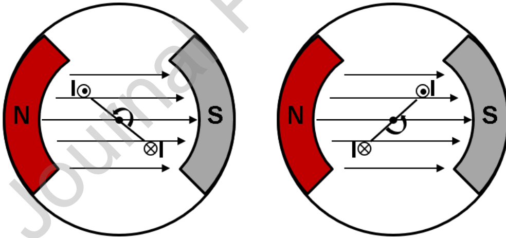
Figure 6: Working mechanism of an electromagnetic harvester: a metal coil cuts through the magnetic induction lines generated by a magnet.
