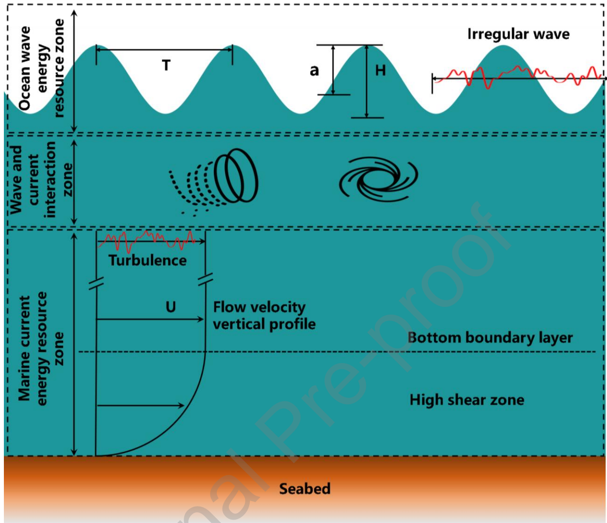
Figure 5: Schematic diagram showing the characteristics and resource zone of OKE.
