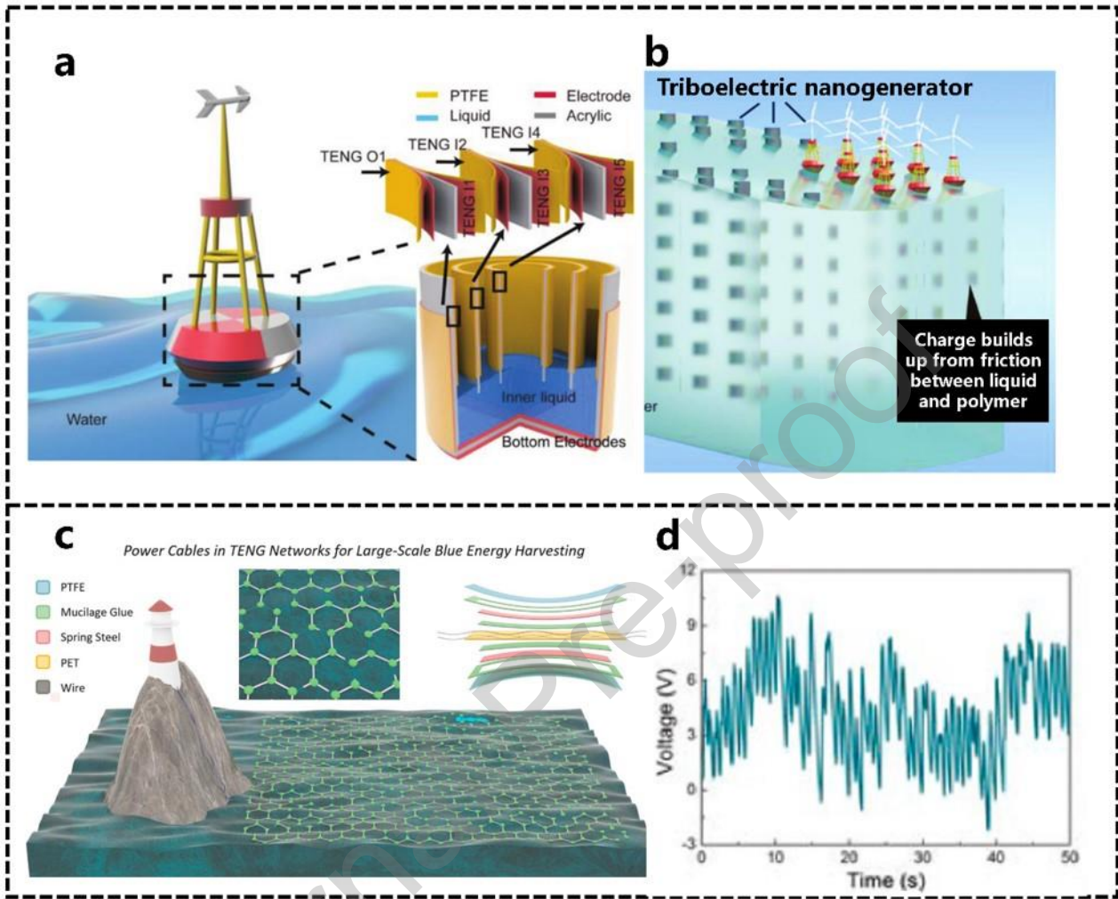
Figure 16: (a) The structure of liquid–solid-contact buoy triboelectric nanogenerators. (b) The schematic illustration of the TENG network which contains thousands of single units. (c) TENGs connected by power cables for large-scale blue energy harvesting with honeycomb-like topology structure. (d) Output voltage of four cables. (a-b) Reproduced with permission from Wiley [200]. (c-d) Reproduced with permission from Elsevier [218].
