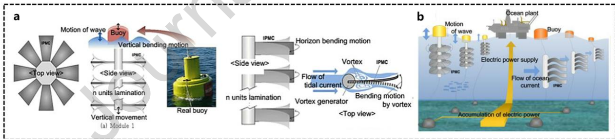
Figure 13: (a) Illustration of a compact movable power system utilizing both vertical wave and horizontal ocean current with a vortex, and (b) schematics of the OKE harvesting structure with the IPMC supplying electricity for stand-alone offshore plants. (a–b) Reproduced with permission from Springer [113].
