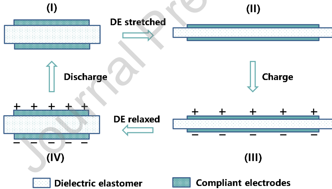
Figure 9: Generating mechanism of DEH.
