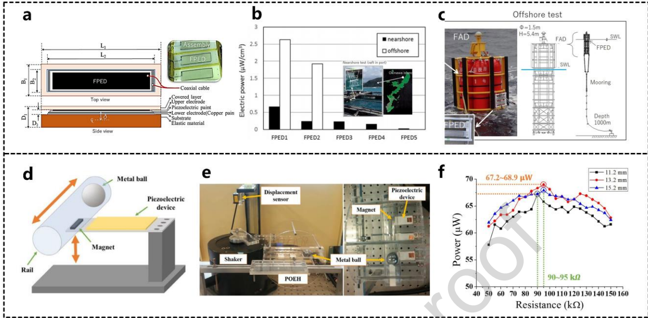
Figure 12: (a) Laminated structure of a FPED painted by spray nozzle. (b) Comparison of electric power generated from each FPED at nearshore and (c) offshore sites. (d) PEH based on sway movement. (e) Test bench construction. (f) Output power of the device for three different shaker displacement values. (a–c) Reproduced with permission from Elsevier [144]. (d–f) Reproduced with permission from Elsevier [145].
