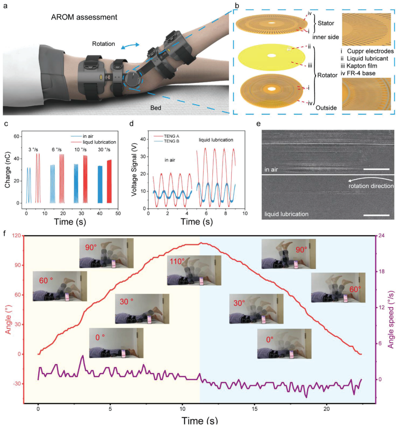
Figure 3. The response of brace angle measurement module. Schematic illustration of a) active range of movement test and b) TENG liquid-enhanced angle sensor with interface liquid enhancement c) Transferred charge of a TENG angle sensor in air and with interface liquid lubrication. d) Open-circuit voltage of TENG angle sensor in air and with interface liquid lubrication. e) SEM images results of Kapton film surface after 100 000 cycles in air and with interface liquid lubrication (scale bar, 100 \mu\text{m} ). f) The real-time angle signals, angle speed, and photos during the active range of movement test.
