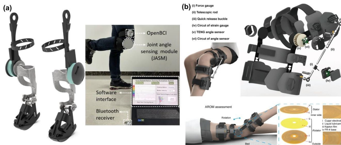
Fig. 13 Scientific rehabilitation. (a) Schematic diagram of a wearable exoskeleton system for the knee joint and the whole system. Reproduced with permission from ref. 45 . Copyright © 2022, American Chemical Society. (b) A perspective view of a brace with a modular device for measuring isometric myodynamia and joint ROM (range of motion). Schematic illustration of active range of movement test and TENG liquid-enhanced angle sensor with interface liquid enhancement. Reproduced with permission from ref. 41 . Copyright 2022 The Authors. Advanced Science published by Wiley-VCH GmbH.
