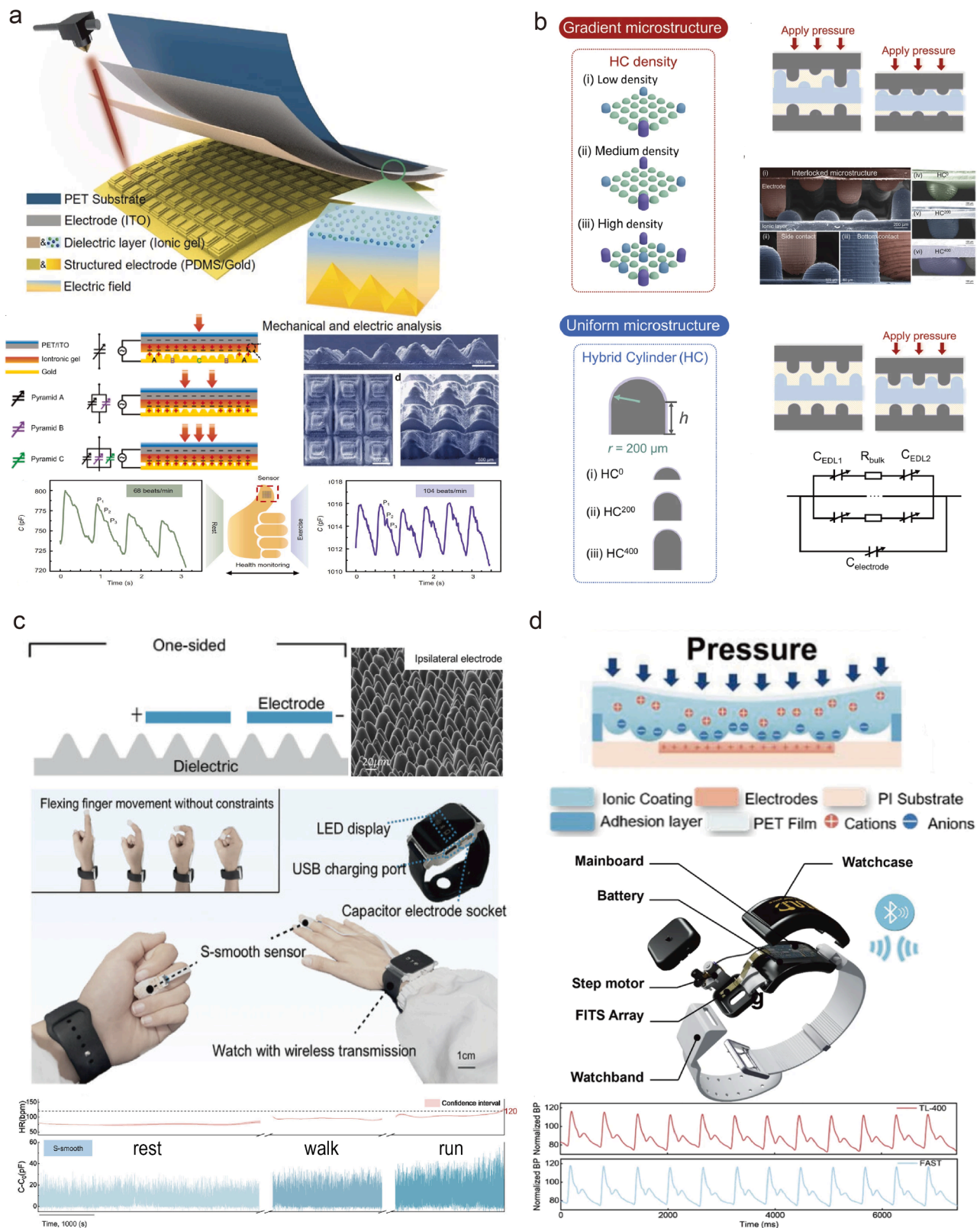
Fig. 5. Flexible capacitive sensors targeting pulse wave monitoring. (a) Programmable iontronic sensor with gradient pyramidal microstructures enabling customizable pressure-response characteristics for broad dynamic range sensing. Reproduced with permission [170]. Copyright 2023, Springer Nature. (b) Schematic illustration of the hybrid cylinders with different heights and different densities. Reproduced with permission [168]. Copyright 2025, Springer Nature. (c) Single-electrode capacitive configuration with low-friction soft-hard interface design for maintaining signal stability during dynamic motion. Reproduced with permission [174]. Copyright 2025, John Wiley and Sons. (d) Closed-loop hemodynamic monitoring system integrating a conformable capacitive sensor array with microfluidic actuation for automatic arterial positioning and optimal contact pressure control. Reproduced with permission [175]. Copyright 2024, Springer Nature.
