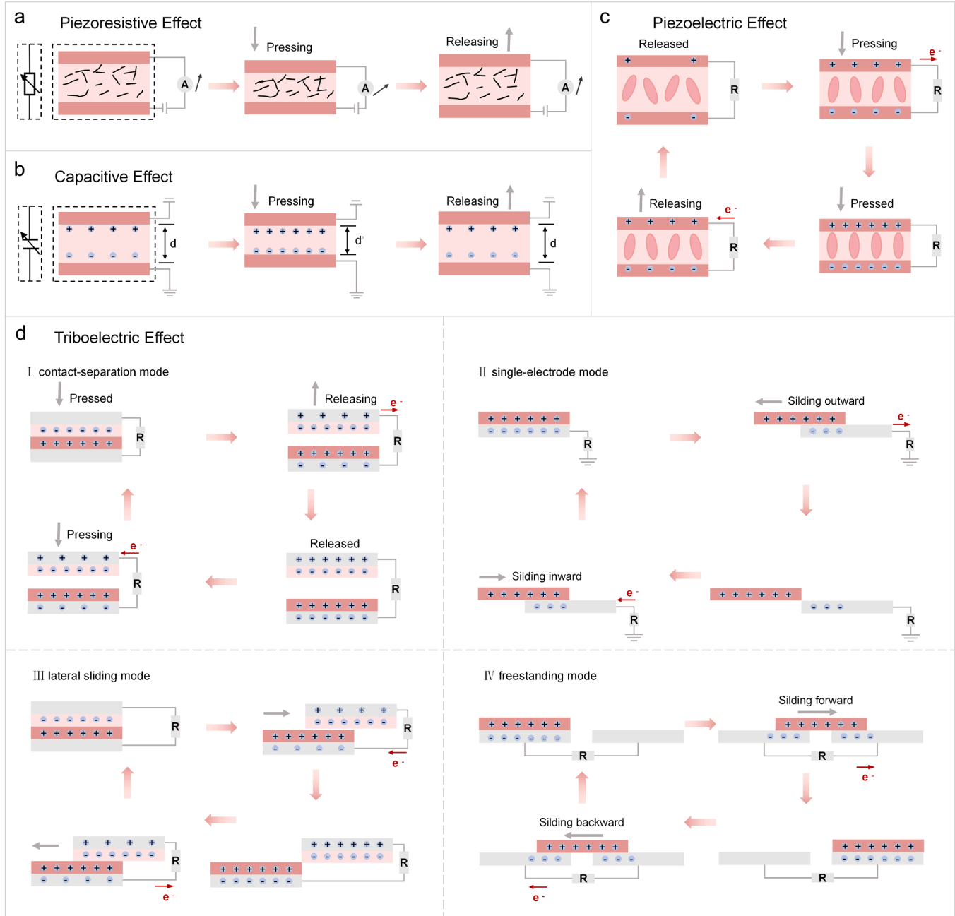
Fig. 2. Schematic illustrations of mechanical transduction mechanisms in wearable pulse wave sensors. (a) Piezoresistive sensing based on deformation-induced changes in electrical resistance. (b) Capacitive sensing based on pressure-induced changes in capacitance. (c) Piezoelectric sensing based on the direct piezoelectric effect, in which applied mechanical stress generates electrical charges. (d) Triboelectric sensing based on contact electrification and electrostatic induction, including four fundamental working modes: (I) contact-separation mode, (II) single-electrode mode, (III) lateral sliding mode, and (IV) freestanding mode.
