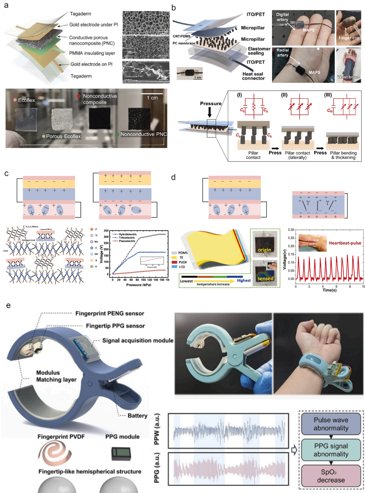
Fig. 8. Hybrid sensors for pulse wave monitoring. (a) Schematic illustration of the porous CNT-Ecoflex foam-based capacitive-resistive hybrid sensor. Reproduced with permission [247]. Copyright 2021, John Wiley and Sons. (b) Device architecture of a microstructure-based capacitive-resistive hybrid sensor. Reproduced with permission [248]. Copyright 2023, Royal Society of Chemistry. (c) Structure and performance of a fiber-based triboelectric-piezoelectric hybrid sensor. Reproduced with permission [249]. Copyright 2025, Elsevier. (d) Schematic of the bio-inspired tribo-piezo-pyro hybrid sensor with an Ag nanowire leaf-venation electrode. Reproduced with permission [250]. Copyright 2018, Elsevier. (e) Schematic of the biomimetic fingertip structure integrating PENG and PPG sensing units. Reproduced with permission [251]. Copyright 2025, John Wiley and Sons.
