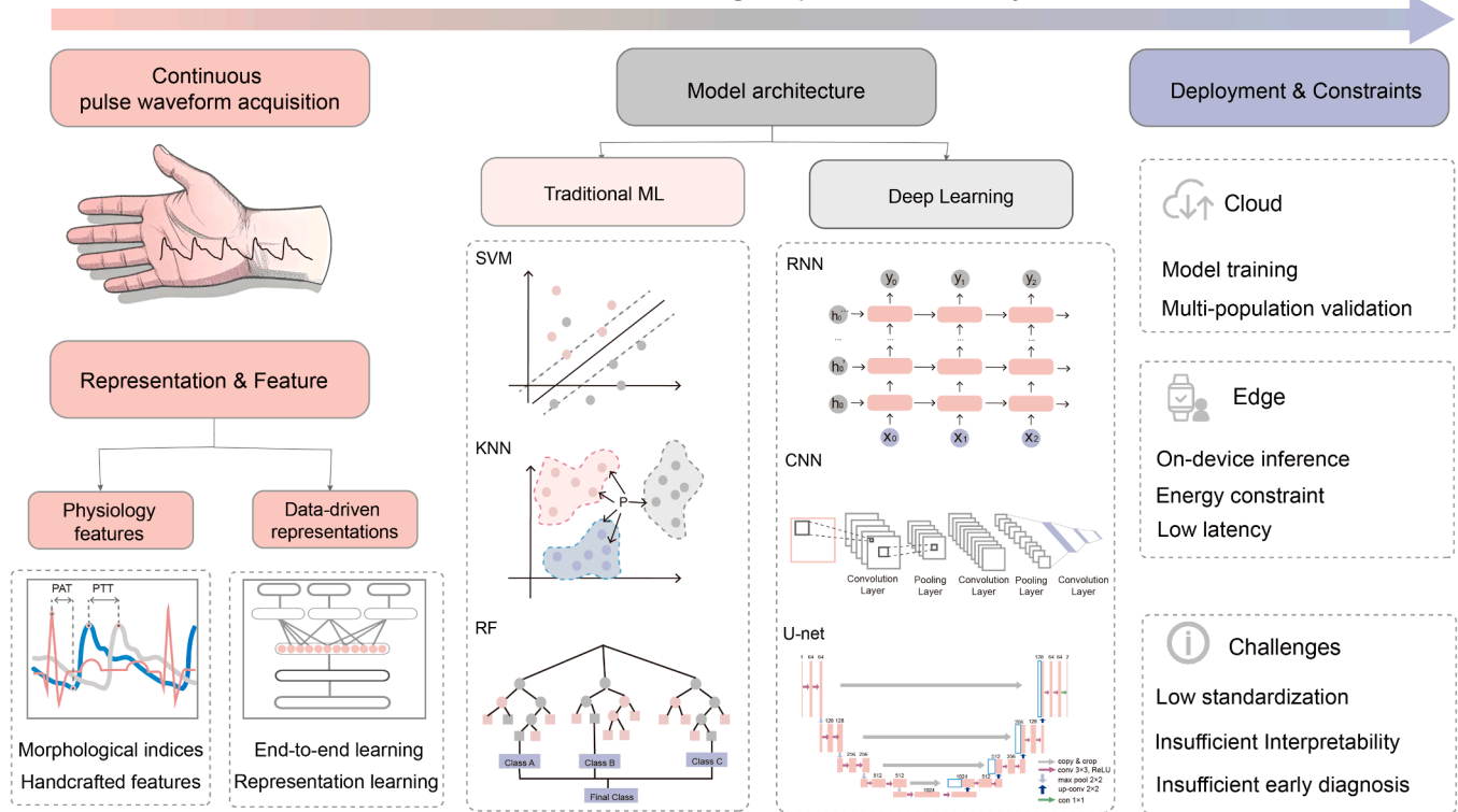
Fig. 10. Panoramic view of machine learning framework for pulse wave analysis.
