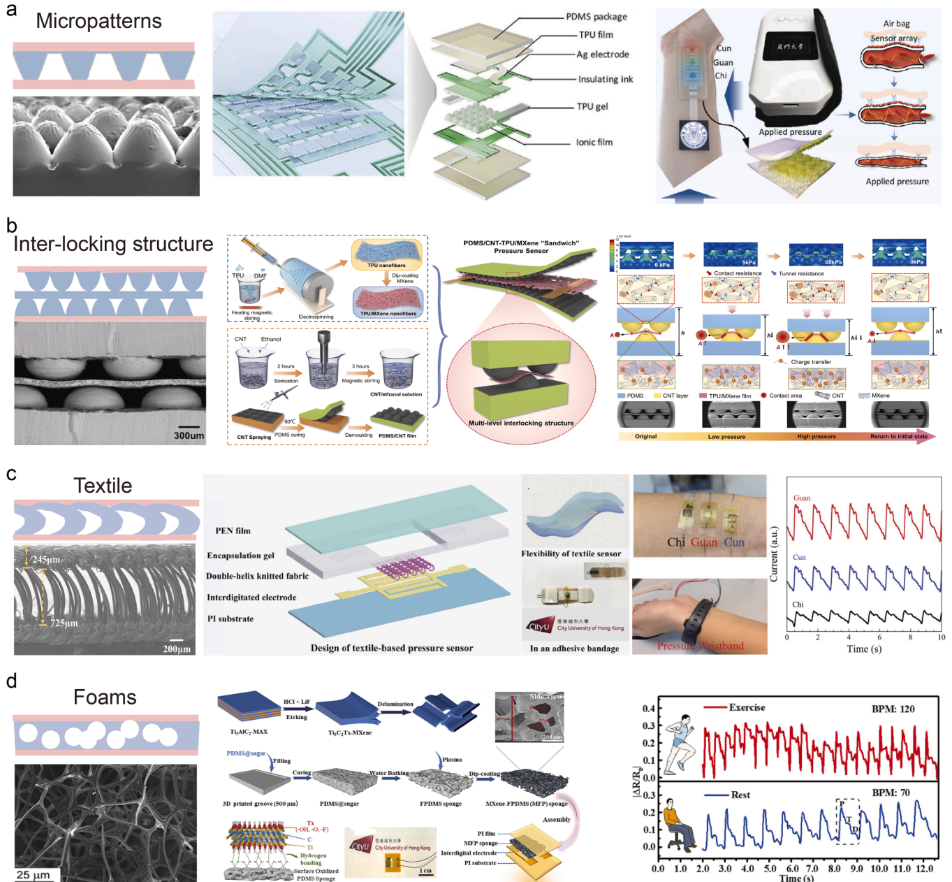
Fig. 4. Advanced piezoresistive sensor designs for pulse monitoring. (a) Dome-structured printed array inspired by TCM pulse diagnosis. Reproduced with permission [131]. Copyright 2024, Springer Nature. (b) Interlocking microdome sandwich with CNT/MXene hybrid network. Reproduced with permission [132]. Copyright 2024, Royal Society of Chemistry. (c) Double-helix yarn textile sensor with ultrafast recovery. Reproduced with permission [133]. Copyright 2021, John Wiley and Sons. (d) Plasma-engineered highly porous MXene/PDMS sponge with hydrogen-bonded interface for enhanced sensitivity and stability. Reproduced with permission from [134]. Copyright 2024, Elsevier.
