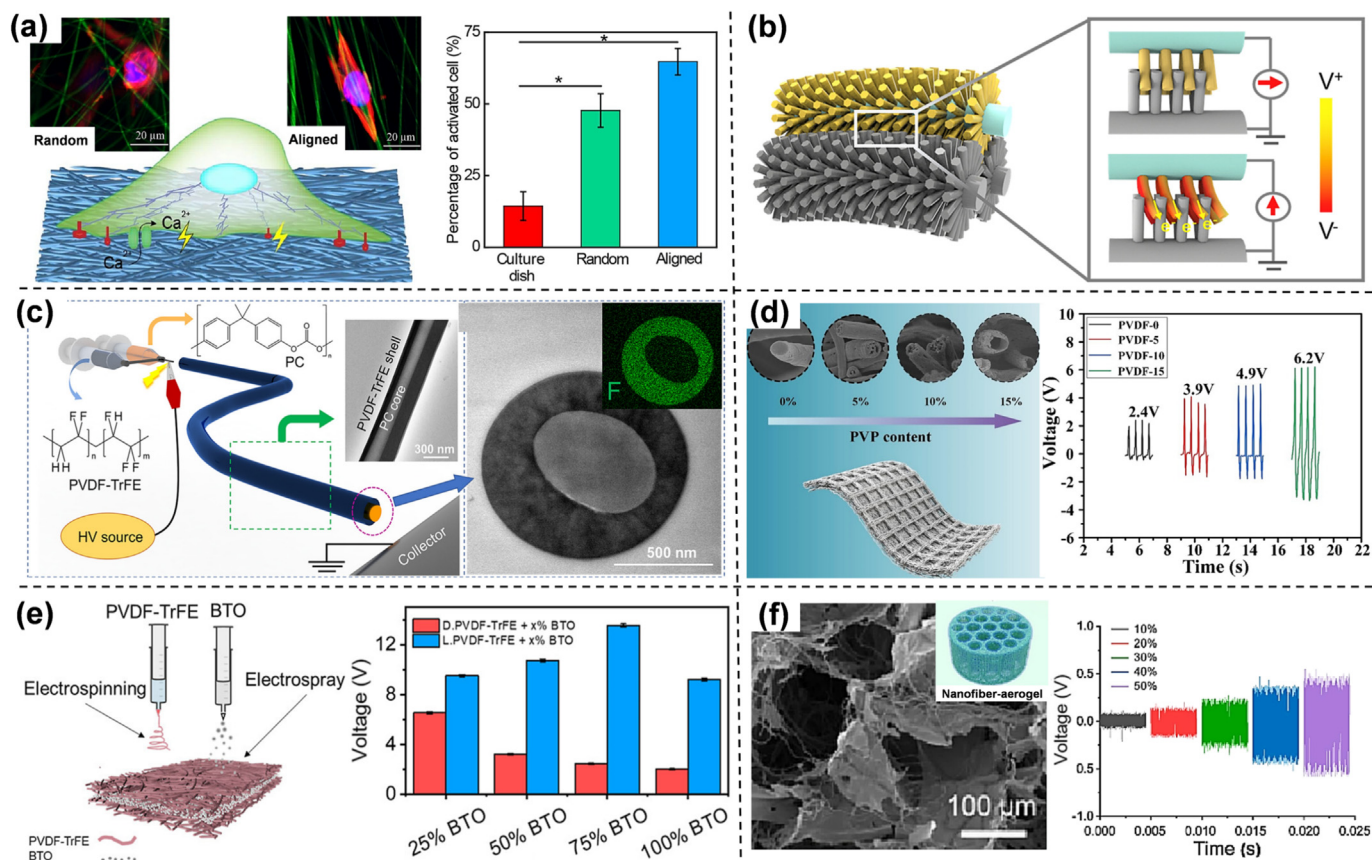
Fig. 3. Different morphologies and microarchitectures of self-enhanced piezoelectric electrospun fibers. (a) Effect of random/aligned fibers on cell morphology and activation state. Reproduced with permission from Ref. [79], Copyright 2021, Elsevier. (b) Schematic diagram of the piezoelectric potential generated on ZnO NRs grown on the fiber surface. Reproduced with permission from Ref. [83], Copyright 2020, Elsevier. (c) PVDF-TrFE nanofibers with a core-shell structure. Reproduced with permission from Ref. [85], Copyright 2023, American Chemical Society. (d) PVDF fibers with different degrees of hollowness and their piezoelectric properties. Reproduced with permission from Ref. [87], Copyright 2024, Elsevier. (e) Electrical output of PVDF-TrFE with different contents of BTO in the sandwich structure. Reproduced with permission from Ref. [88], Copyright 2023, American Chemical Society. (f) The morphology of 3D porous scaffolds and electrical output at different US frequencies. Reproduced with permission from Ref. [90], Copyright 2023, Elsevier.
