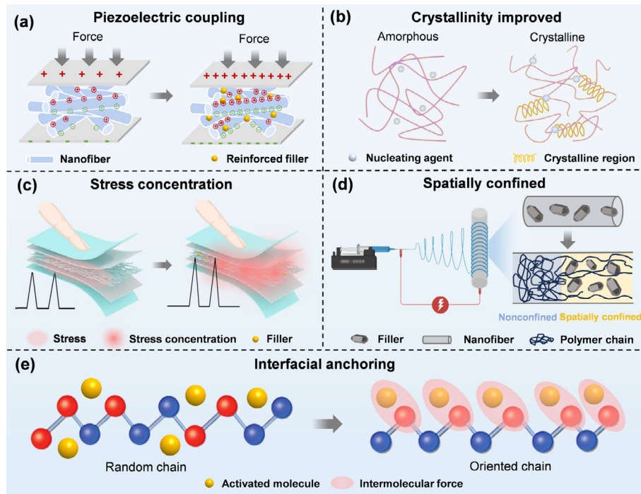
Fig. 4. Enhancement strategies for the piezoelectric property of electrospun fibers. (a) Piezoelectric effect coupling; (b) crystallinity improvement; (c) stress concentration amplifying the piezoelectric effect; (d) spatially confined effect; (e) interfacial anchoring enhancement strategy.
